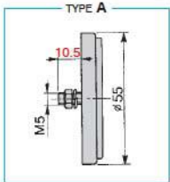
Catadiottri ø 55 mm. CON VITE Reflex reflectors ø 55 mm. WITH SCREW
